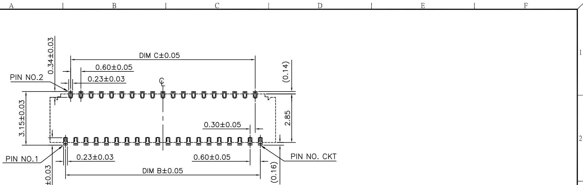
RECOMMENDED P.C.B. LAYOUT HATCHED AREA SHOWS SOLDERING LAND. (GENERAL TOLERANCE: ±0.05mm)
