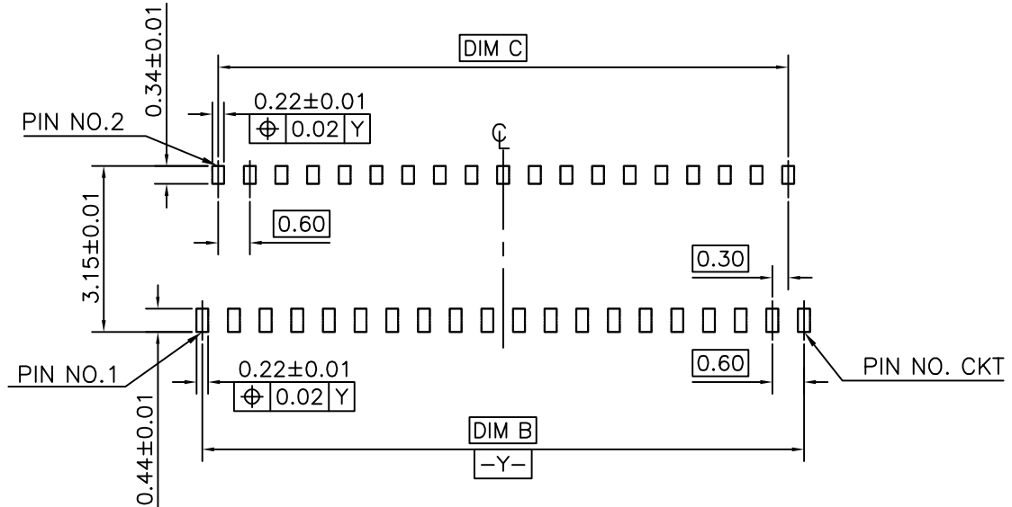
RECOMMENDED STENCIL PATTERN (RECOMMENDED STENCIL THICKNESS t=0.12mm)
